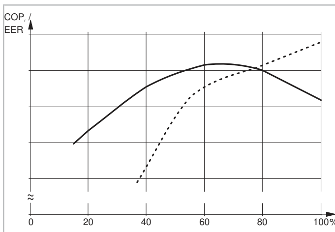
Fig. 2: Comparison of the capacity control efficiency characteristics of screw compressors with slider control vs. frequency inverter (FI): coefficient of performance COP r /EER (ratio of refrigerating capacity to power absorbed) as a function of the load.
