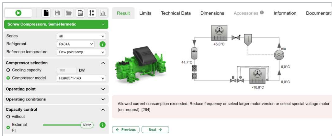
Fig. 8: By increasing the operating frequency of the selected compressor, the maximum current consumption may be exceeded. In this case, the software recommends a larger motor version or a special voltage motor.
