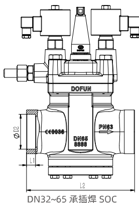
两步开启电磁阀 Two-Step Open Solenoid Valve
